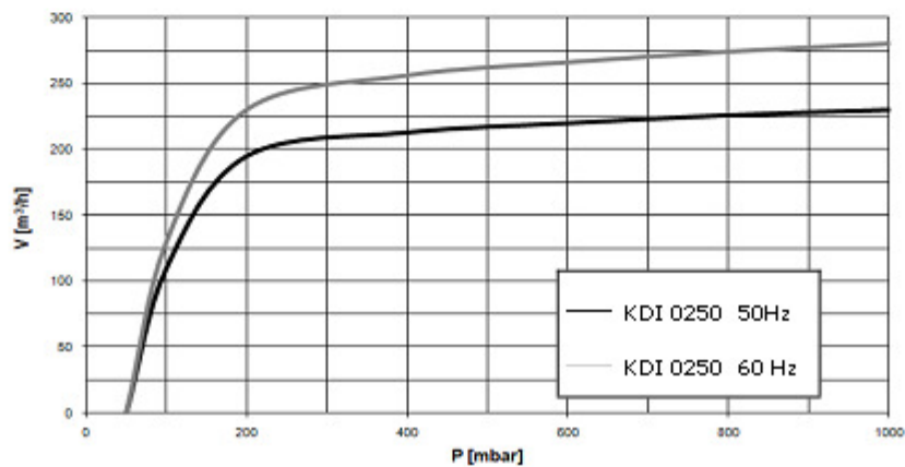
Pumping speed curve
