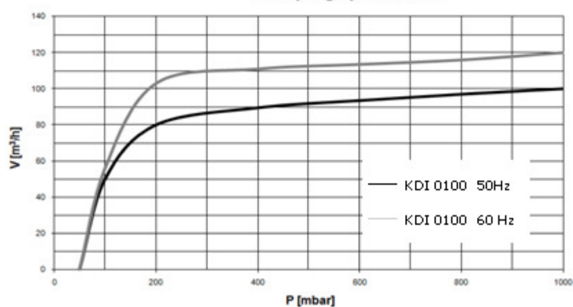
Pumping speed curve
