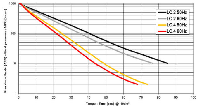
NOTE: Graph shows inlet pressure at a temperature of 20°C (tolerance ±10%)
